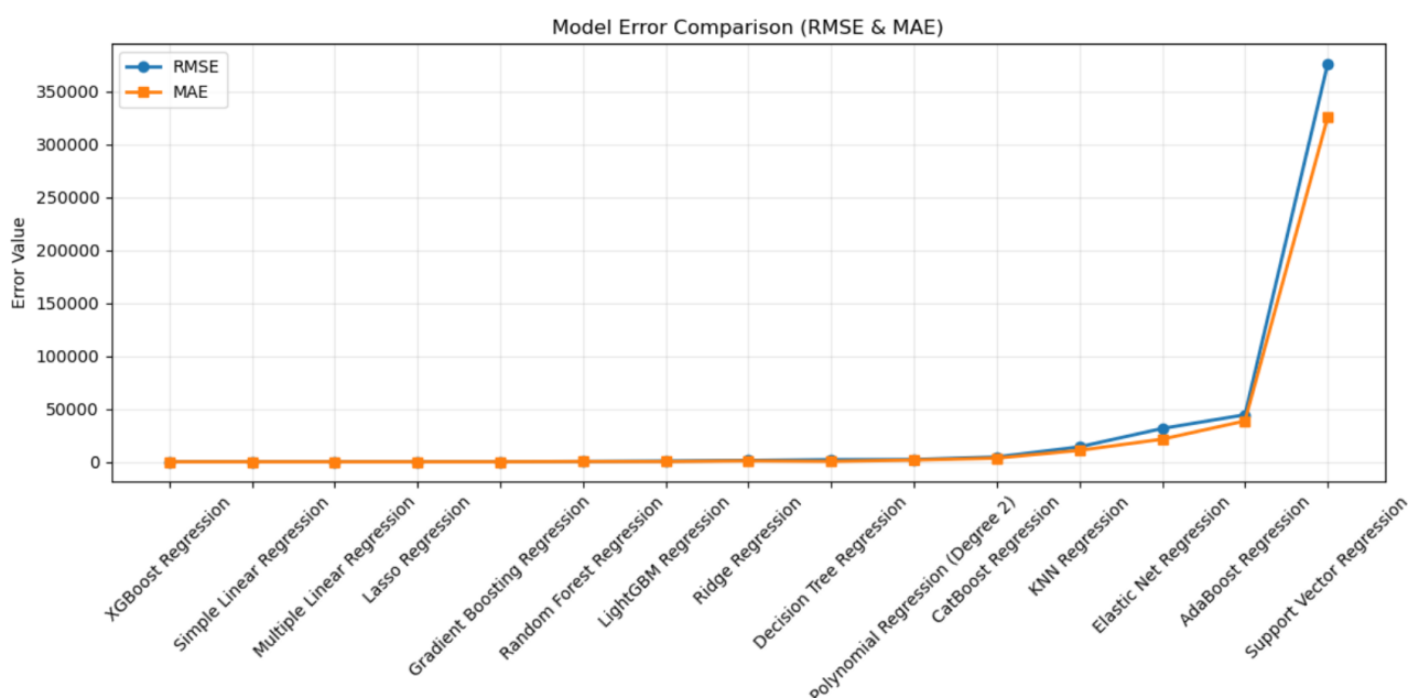
Fig. 3. RMSE and MAE comparison of ML models
